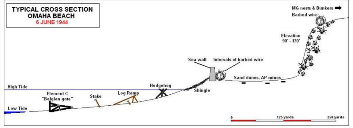
Element C or the Belgian Gate was designed to destroy landing craft as they were submerged at high tide
